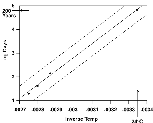
Figure 2 Bivariate Fit of Log Days by Inverse Temp
