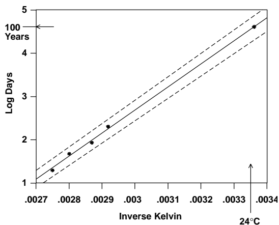
Figure 1 Four-Point Prediction
